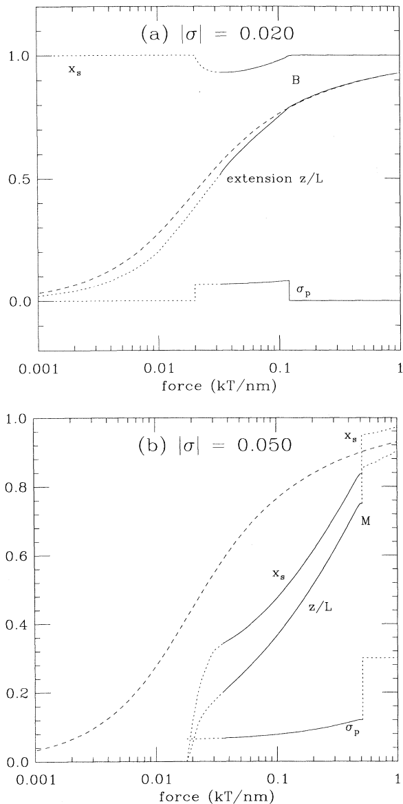
FIG. 8. Extension versus force for DNA with fixed linking number (note 1 k_B T / \text{nm} \approx 4 \times 10^{-12} \text{N} ). The \sigma = 0 calculation (dashed curve) is exact while the other curves are calculated in the large-force limit; that Gaussian calculation is in error by \geq 5\% for extensions z/L < 0.5 and 0.25 for |\sigma| = 0.02 and 0.05 , respectively, and below these limits expected behaviors are dotted. A plectonemic bubble appears with decreasing force at point B for |\sigma| = 0.02 . For |\sigma| = 0.05 the concentration of link in the plectonemic region causes the DNA to unwind or melt at point M as force increases; results beyond M are dotted, since they depend on poorly known details of melted DNA.
