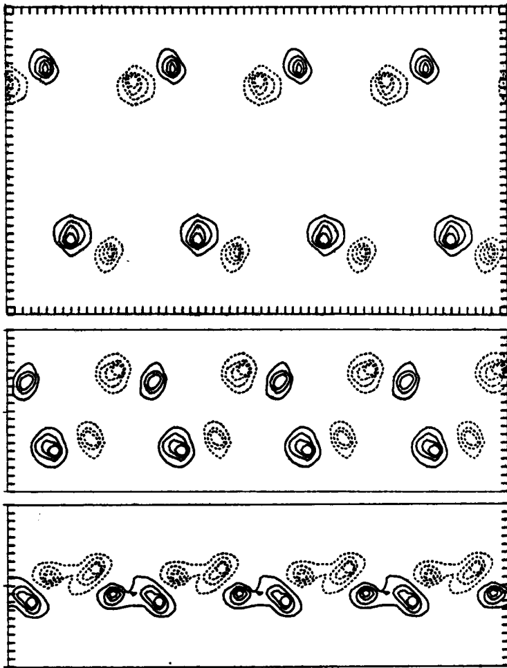
FIGURE 10. Continuation of figure 9. The bottom two panels were produced much wider by the plotting routine, indicating that vortex 'debris' was left behind (§2). The magnitude of this vorticity was less than the lowest vorticity contour level, and the panel was reduced in size for reproduction.
